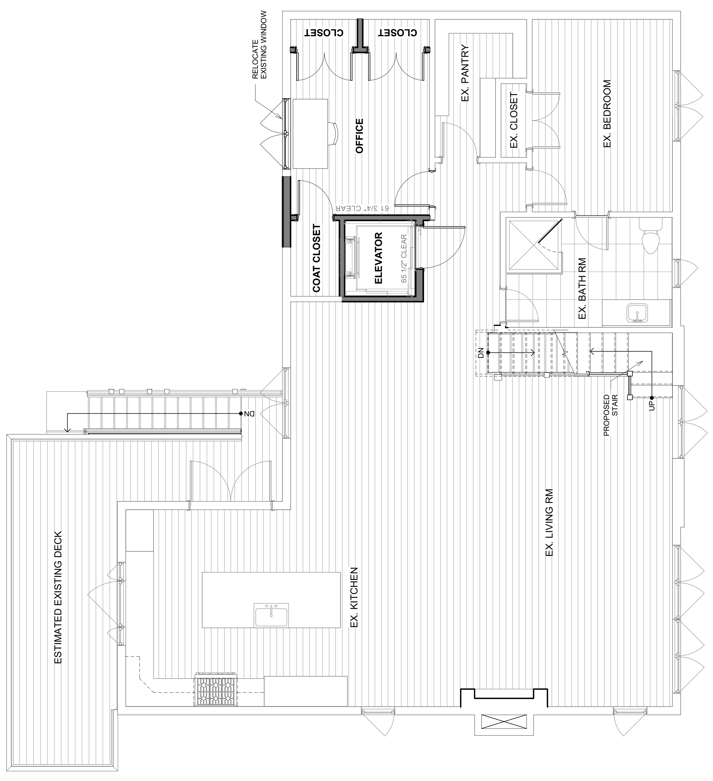
② PROPOSED FIRST FLOOR 1/4" = 1'-0"
