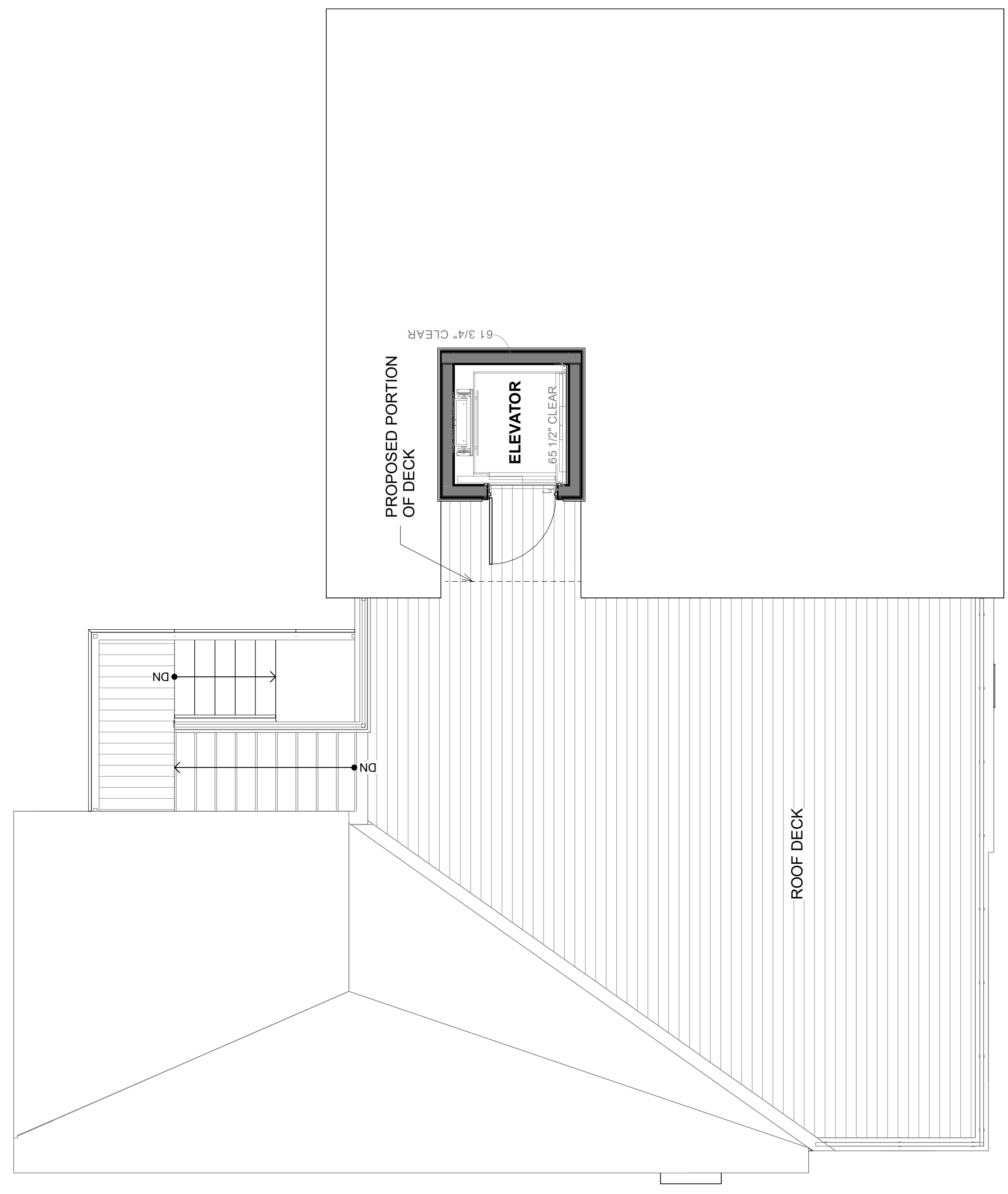
② PROPOSED ROOF DECK 1/4" = 1'-0"
