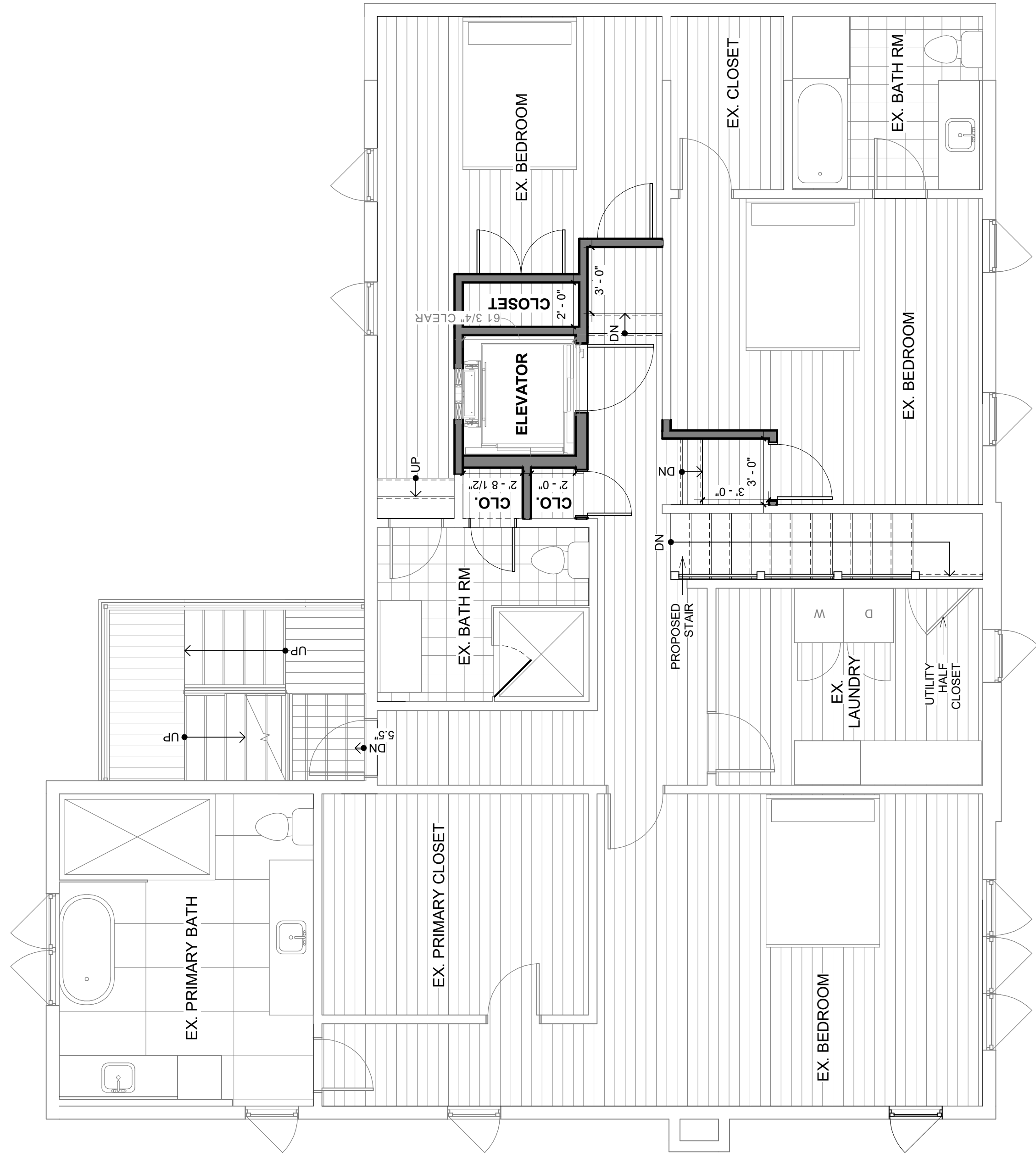
① PROPOSED SECOND FLOOR 1/4" = 1'-0"
