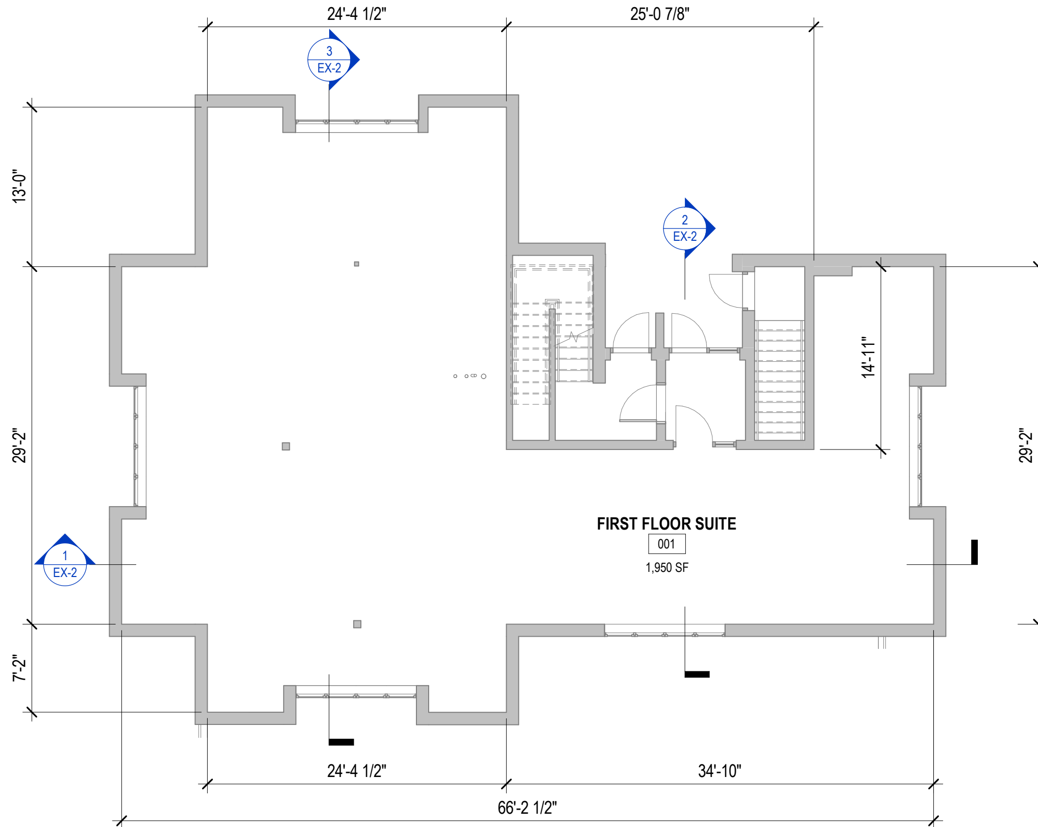
1 EXISTING FLOOR PLAN - LEVEL 1 1/8" = 1'-0"
