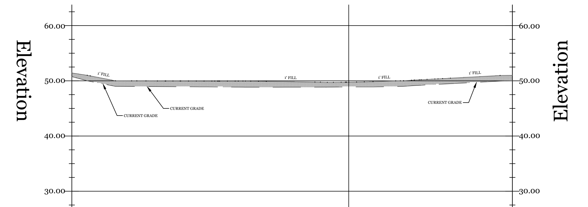
PROFILE OF REDISTRIBUTION AREA 2 ALIGNMENT 1 VERT. SCALE: 1" = 10' HORIZ. SCALE: 1" = 20'
