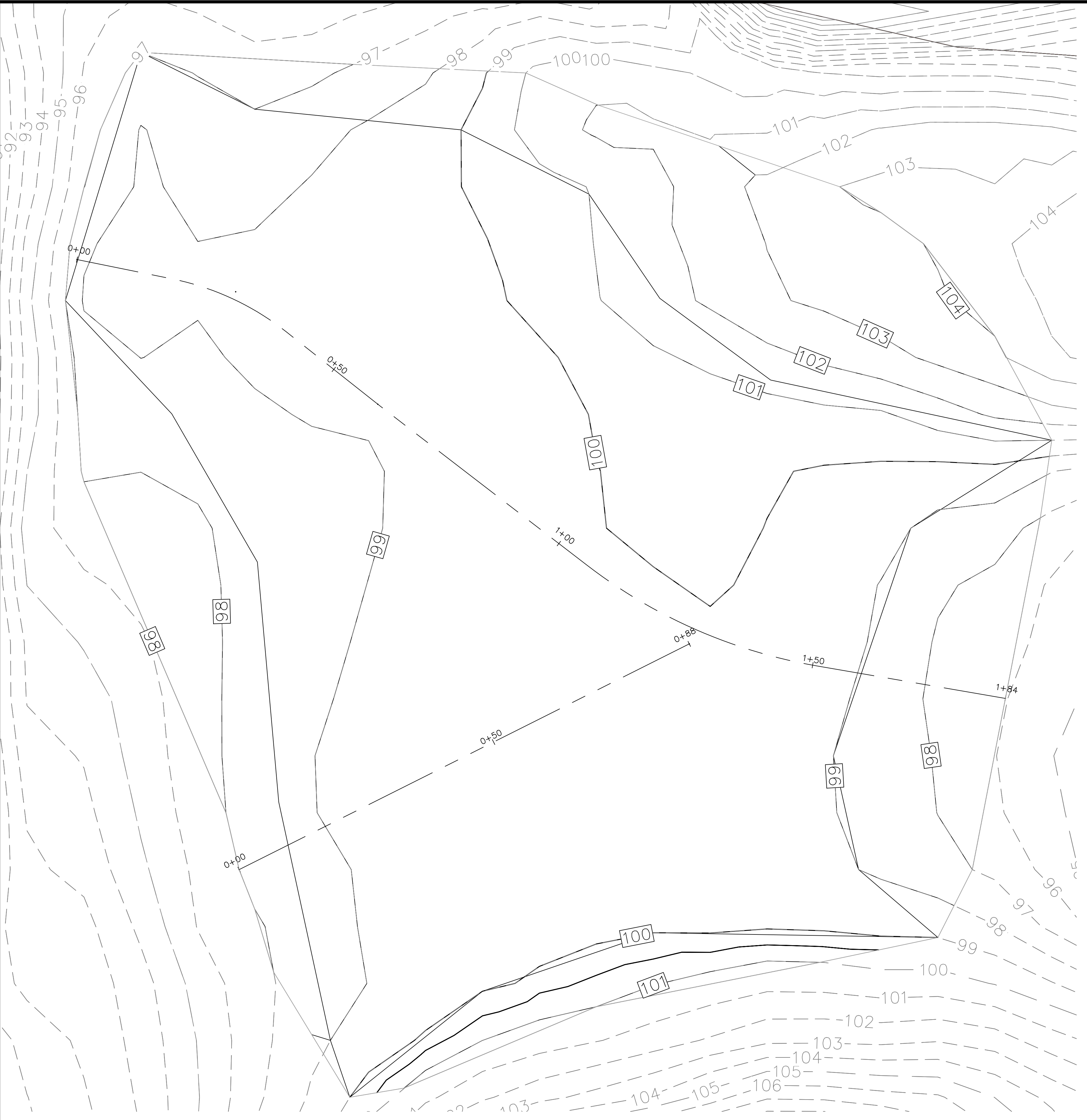
REDISTRIBUTION AREA 1 SCALE: 1"=10'
