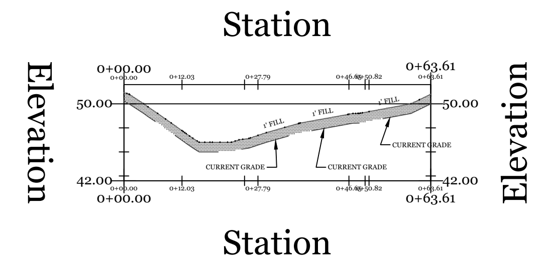
PROFILE OF REDISTRIBUTION AREA 2 ALIGNMENT 2 VERT. SCALE: 1" = 10' HORIZ. SCALE: 1" = 20'
