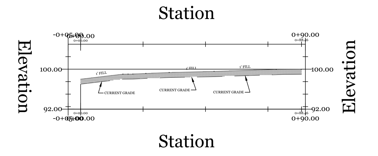
PROFILE OF REDISTRIBUTION AREA 1 ALIGNMENT 2 VERT. SCALE: 1" = 10' HORIZ. SCALE: 1" = 20'
