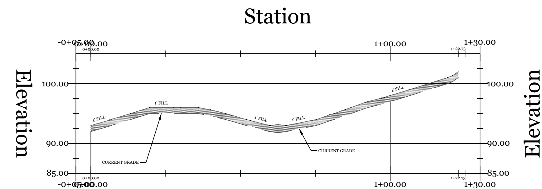
PROFILE OF REDISTRIBUTION AREA 4 ALIGNMENT 2 VERT. SCALE: 1" = 10' HORIZ. SCALE: 1" = 20'
